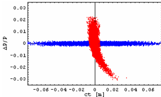
Figure 5: Longitudinal phase space of injected beam at injection (blue) and after 48 turns (red).
