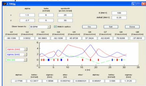
Figure 2: Optics control GUI for the LTB
