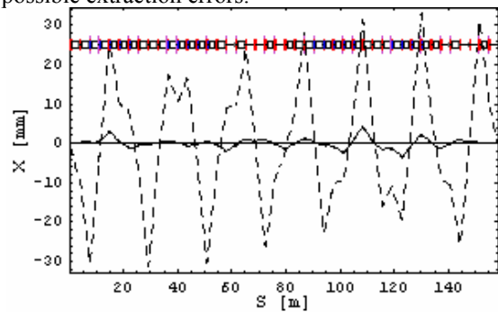
Figure 3: Closed orbit distortion for sorted dipole magnets (solid line) and worst-case (dashed line) error distributions in the booster
