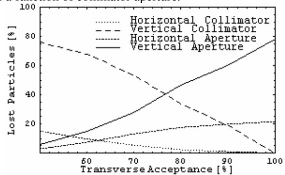
Figure 4: Percentages of total particle losses occurring at the collimators ("collimator") and elsewhere in the storage ring ("aperture") as a function of the relative transverse acceptance: 100% means collimator wide open, 50% means 12.2 mm in H and 4.5 mm in V half apertures.
