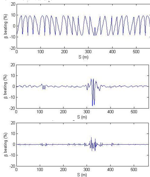
Figure 6: Compensation of \beta -beat with LOCO. Vertical \beta -beat without compensation (top), vertical \beta -beat with compensation (middle), horizontal \beta -beat with compensation (bottom).
