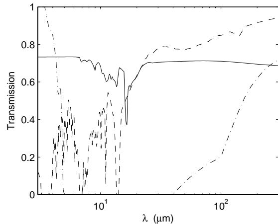
Figure 2: Transmission of possible vacuum windows for THz radiation. Fused silica (---), High-density polyethylene, (- - -) Silicon (—), each with a thickness of 1.5\ \text{mm} .
