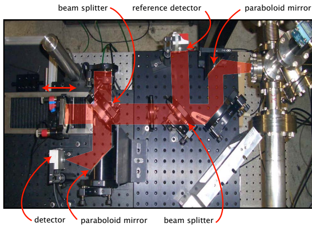
Figure 1: The scanning Michelson interferometer, used to measure the length of the electron bunches in the FFTB.
