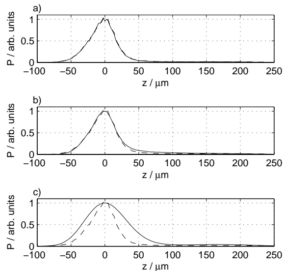
Figure 3: Effect of the window transmission on the shape of the radiation pulse: original pulse (---) and transmitted pulse (—). a) Fused silica (quartz) b) High-density polyethylene, and c) Silicon.
