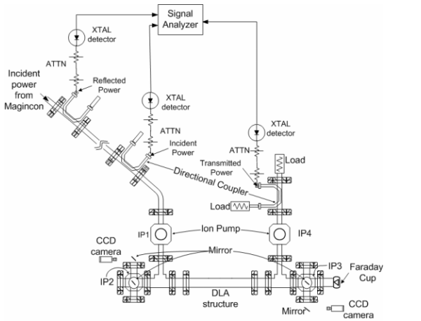
Figure 2: Experimental setup used to test DLA structures with high power RF.
