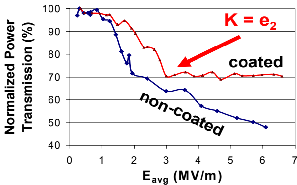
Figure 3: Comparison of the transmitted power for the coated and non-coated alumina-based DLA structures. Saturation occurs when the impact energy (K) is greater than the second crossover energy ( e_2 ).
