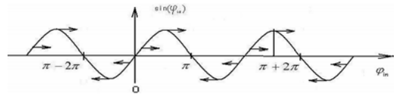
Figure 2: In the EOC scheme electrons are grouping near the phases \varphi_{in} = \pi + 2\pi m (energies E_m ).
