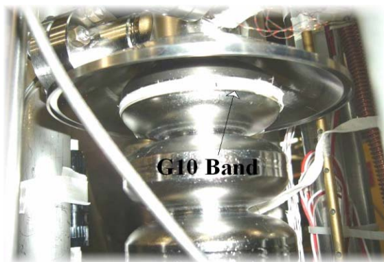
Figure 2: Cernox RTD thermometry G10 band wrapped around the cavity equator.
