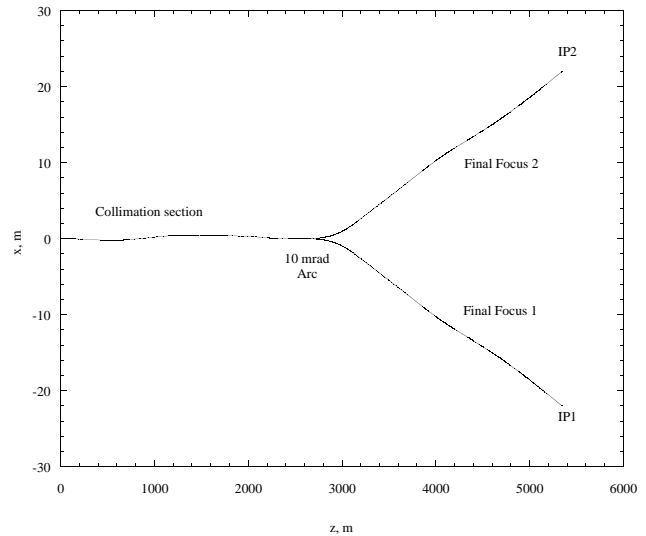
Figure 1: Schematic of NLC Beam Delivery System.
