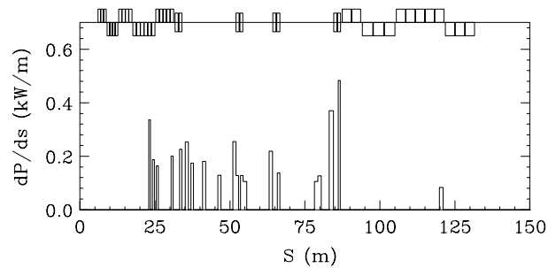
Figure 5: Distribution of the beam power loss.
