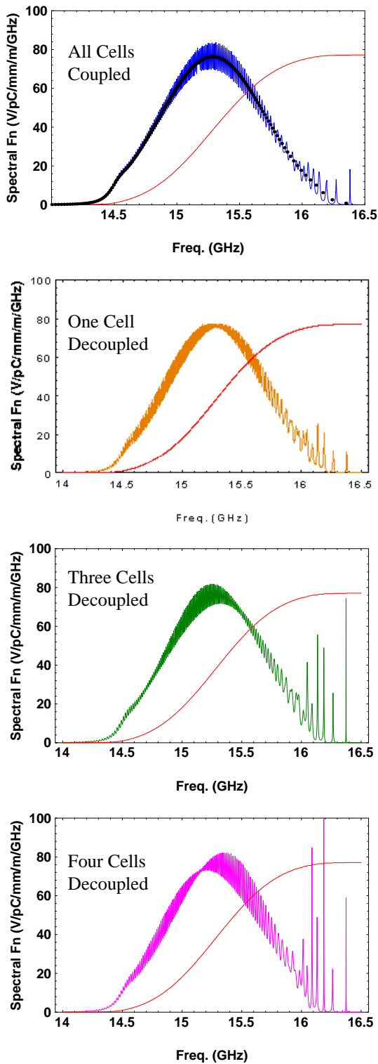
Figure 2: Uppermost is the spectral function for all cells coupled (where the dots indicate the smoothed undamped spectral function). The subsequent curves are computed for 1 cell decoupled, followed by three, and four cells (lowermost) decoupled from both the upstream and downstream end of the RDDS
