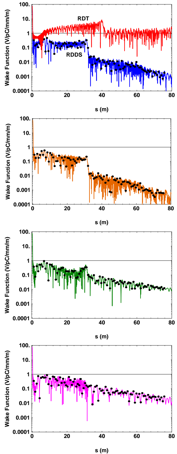
Figure 3: Uppermost is shown a comparison of the RDDS versus the RDT (Rounded Detuned, see main text) wake function for all cells coupled. The subsequent curves are computed for 1 cell decoupled, three, and finally 4 cells (lowermost) decoupled from both the upstream and downstream end of the RDDS.
