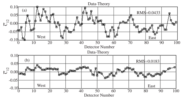
Figure 3. \bar{C}_{12} at each detector around the ring measured (a) before and (b) after the quadrupoles were leveled. The rms. value is 4.3% before and 1.8% after the quadrupoles were aligned [6].
