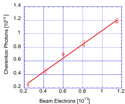
Figure 4: Photon yield vs. number of electrons.
