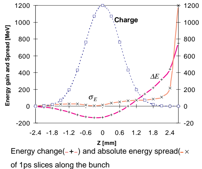
Figure 2: Simulated time resolved measurements.
