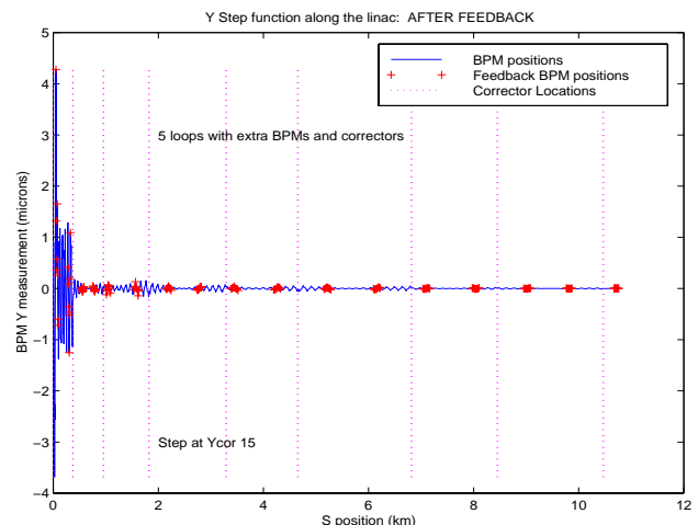
Fig 4: Linac Orbit with Improved Feedback Configuration
