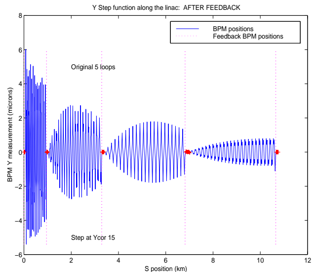
Fig 3: Linac Orbit with Original Feedback Configuration
