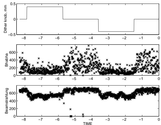
Fig 1: Dithering Process for Luminosity Optimization Feedback
