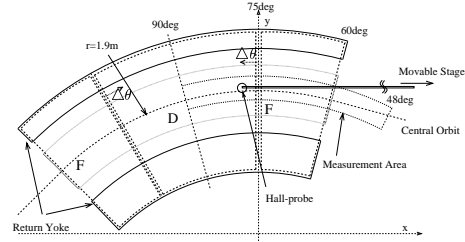
Figure 3: Geometry of the measurement
