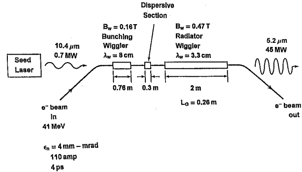
Figure 1: schematic diagram of the HGHG experiment
