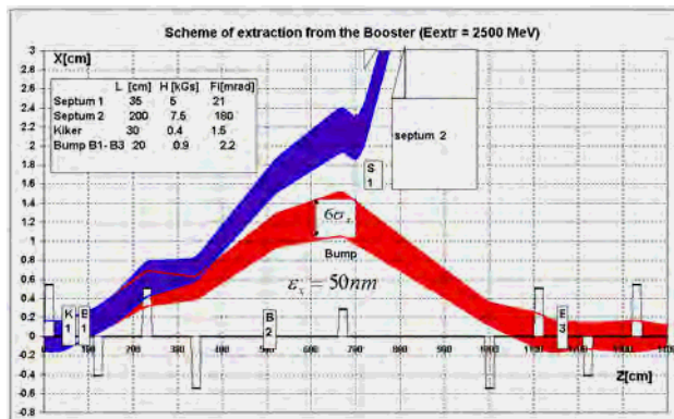
Figure 8: Extraction scheme
