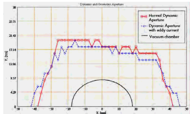
Figure 5: Dynamic aperture
