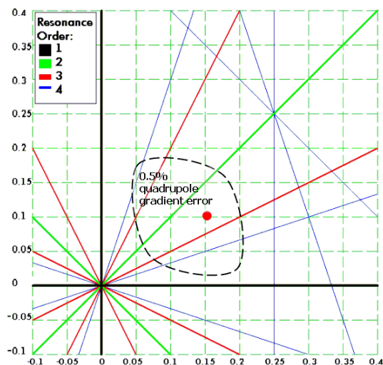
Figure 6: Tune diagram
