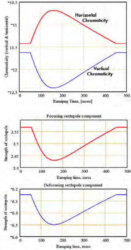
Figure 4. Change of the chromaticity and sextupole magnets' strength during ramping.
