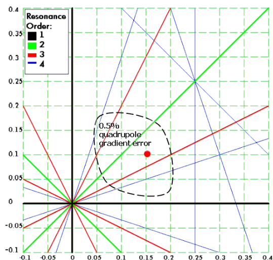
Figure 6. Tune diagram.
