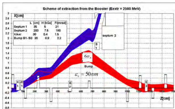
Figure 8. Extraction scheme.
