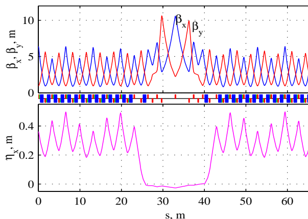
Figure 2: Optical functions.
