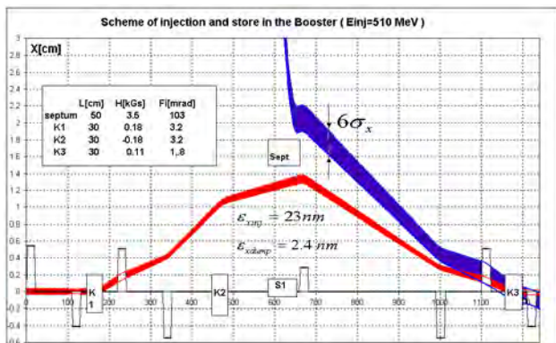
Figure 7. Injection scheme.
