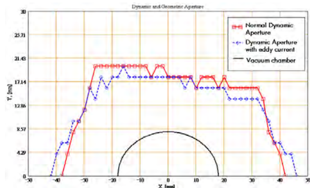
Figure 5. Dynamic aperture.
