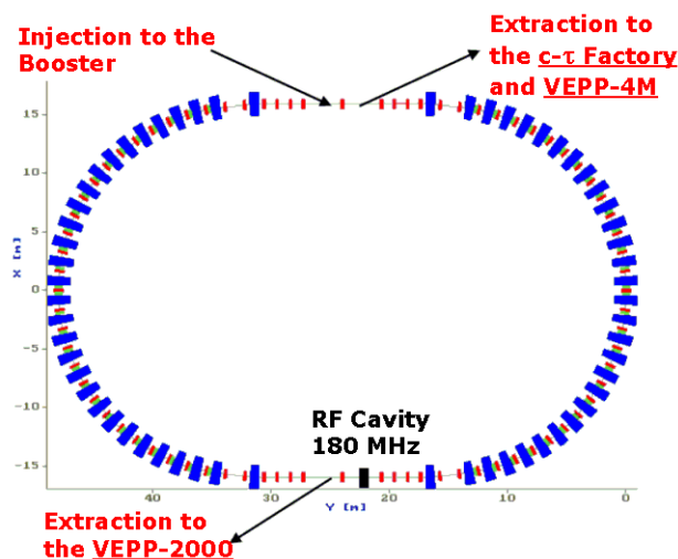
Figure 1: Layout of the synchrotron.
