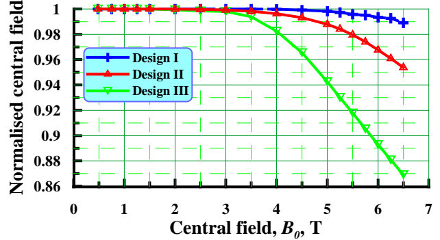
Fig. 4: Normalised field versus central field B_0 .
