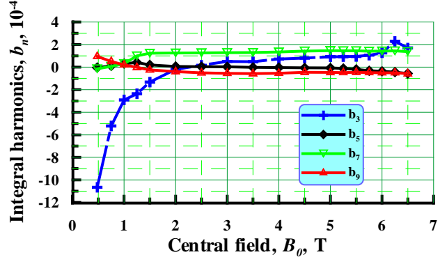
Fig. 5: Integral field harmonics in design I versus B_0 .
