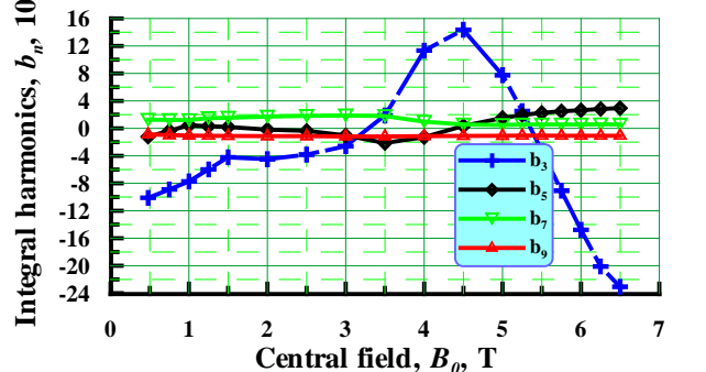
Fig. 7: Integral field harmonics in design III versus B_0 .
