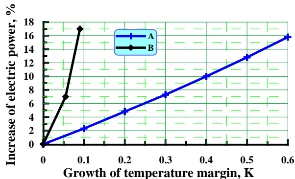
Fig. 8: Dependence of electric power increase for liquid helium production by SIS300 cryogenic system on growth of temperature margin for SIS300 dipole (Design III): A is reduction of liquid helium temperature below
