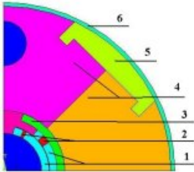
Fig. 3: Design III: 1 – coil; 2 – wedge; 3 – spacer; 4 – iron yoke; 5 – C-clamp; 6 – outer shell.
