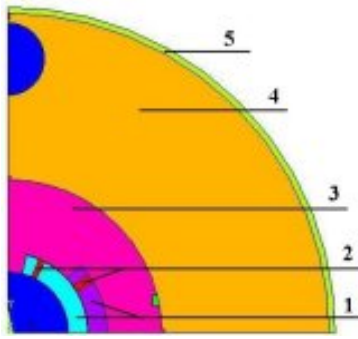
Fig. 1: Design I: 1 – coil; 2 – wedge; 3 – collars; 4 – iron yoke; 5 – outer shell; 6 – staple.
