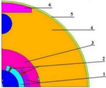
Fig. 2: Design II: 1 – coil; 2 – wedge; 3 – collars; 4 – iron yoke; 5 – outer shell; 6 – clamp.
