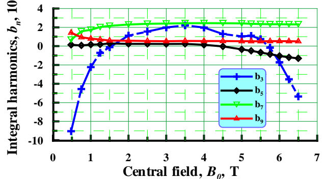
Fig. 6: Integral field harmonics in design II versus B_0 .
