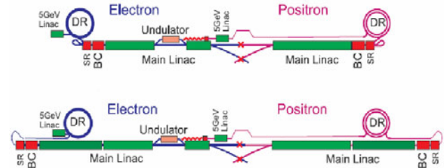
Figure 1: Two stages of the project. 500 GeV machine (top), after increasing - 1TeV stage (bottom).
