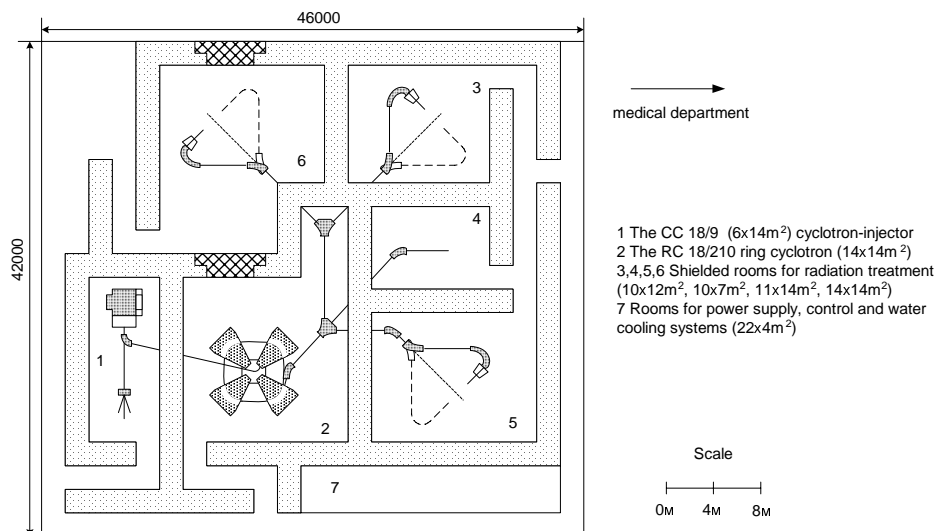
Figure 2: The system for proton therapy. Layout of the equipment.
