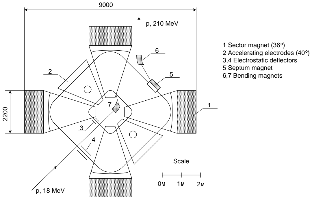
Figure 1: The RC-18/210 ring cyclotron
