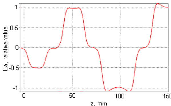
Figure 2: Distribution of electric field in accelerating structure.
