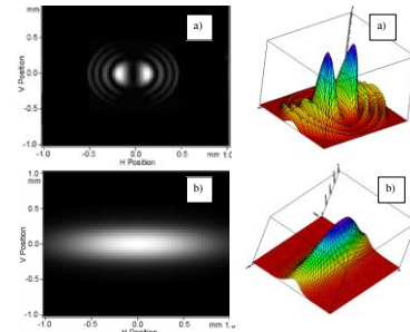
Figure 4: Distribution of flux density for second harmonic a) \epsilon_{x0}=\epsilon_{z0}=0 , \Delta E/E=0 ; b) \epsilon_{x0}=4.9 nm-rad, \Delta E/E=5 \cdot 10^{-4} .
