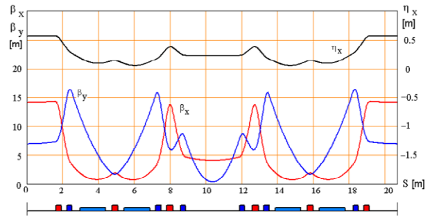
Figure 1: Optical function of storage ring SIBERIA-2 with \epsilon_{x0} = 18 nm-rad at E=2.5 GeV.
