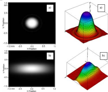
Figure 3: Distribution of flux density for first harmonic a) \epsilon_{x0}=\epsilon_{z0}=0 , \Delta E/E=0 ; b) \epsilon_{x0}=4.9 nm-rad, \Delta E/E=5 \cdot 10^{-4} .
