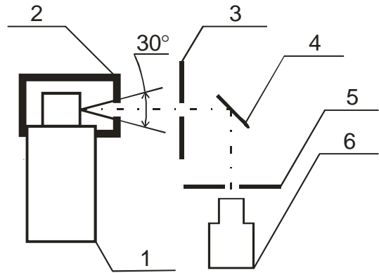
Figure 4: Equipment layout.
