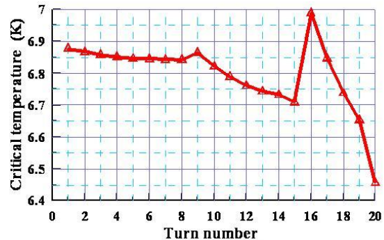
Figure 5: Critical temperatures in turns.
