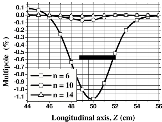
Figure 3: Multipoles b_6 , b_{10} , b_{14} along longitudinal axis.
