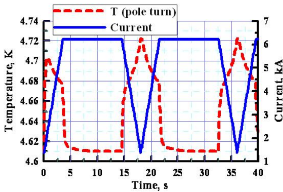
Figure 6: Change temperature in the last turn of magnet and current during SIS 300 cycles.
