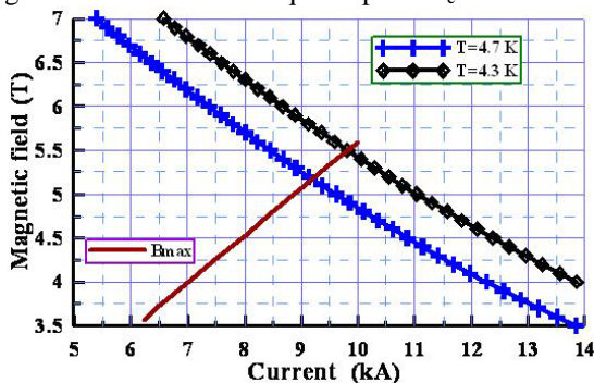
Figure 4: Dependences of maximal field in coil on operating current and critical current of cable on magnetic field.
