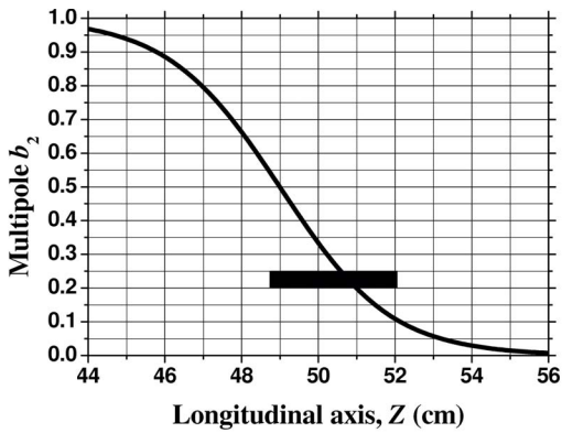
Figure 2: Multipole b_2 along longitudinal axis.
