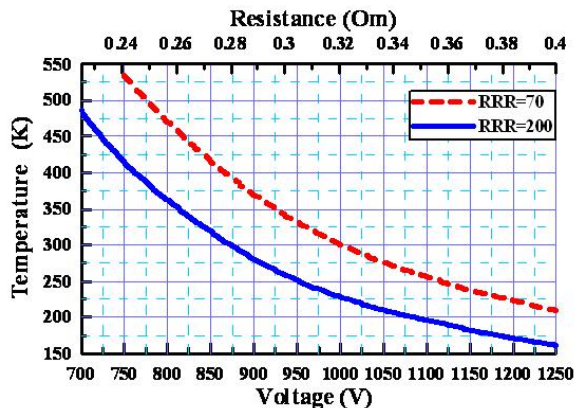
Figure 7: Maximum temperature in the coil as function of dump resistor resistance and voltage to ground for RRR = 70 (dotted line) and 200 (solid line).
