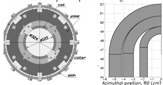
Figure 1: General view of the quadrupole cross section (left) and involutes of the end part (right).
