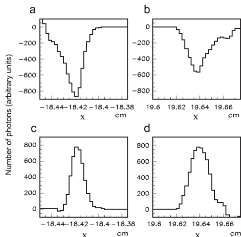
Fig. 6 Simulated differences of SR spectra versus the x-coordinate close to the right (a) and (c) and left (b) and (d) fan edges at the electron energies of 250 GeV and 250 \pm 0.025 GeV.
