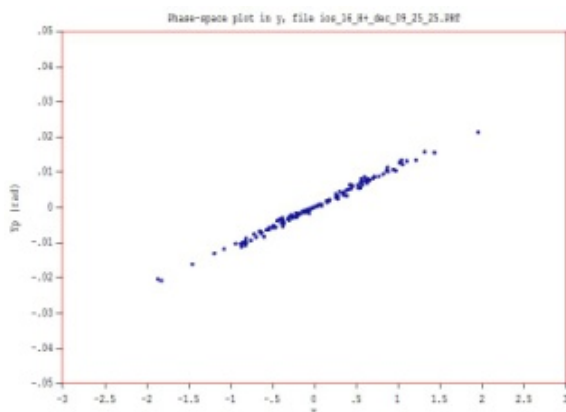
Figure 3: Results of an ion beam simulation with TRAK code. Phase space portrait of the ion beam at distance of 200 cm from the accelerating tube output.
