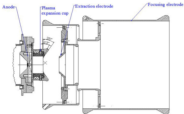
Figure 1: The ion beam formation system of the duoplasmatron.
