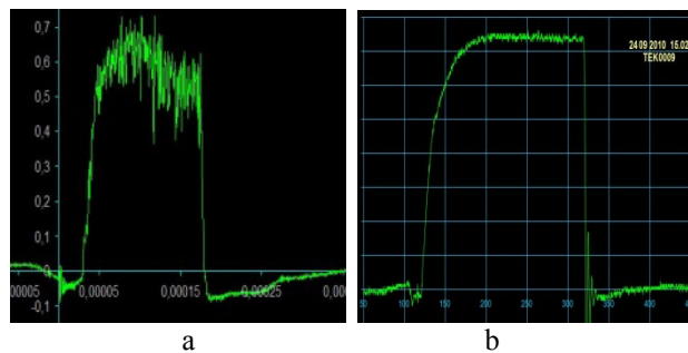
Figure 4: Oscillograms of the ion beam at the injector output, a) gridless ion beam formation system b) new ion beam formation system
