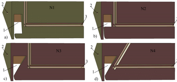
Figure 2: Different options for vane undercuts and cooling channels. 1 - vane undercuts, 2 - the channels for cavity body cooling, 3 - the vane channel.
