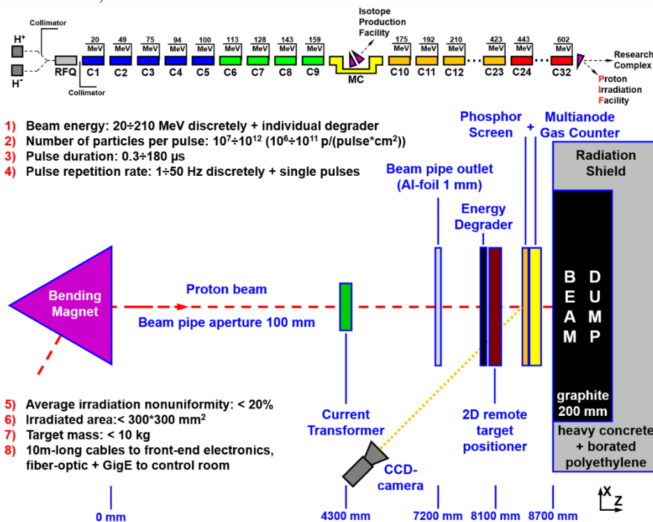
Figure 1: General layouts of the linac and proton irradiation facility at the outlet of the linac.
