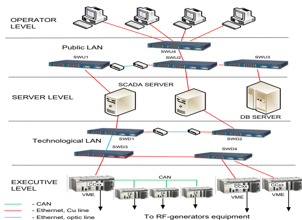
Figure 2: Structure of RF-generators CS.
