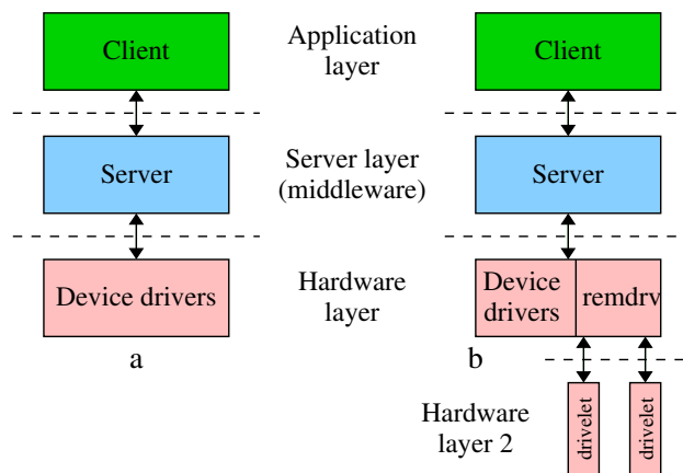
Figure 1: (a) Classic 3-layer architecture; (b) CX with 2-part hardware layer.
