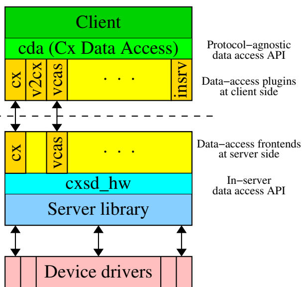
Figure 2: CXv4 core modular structure.
