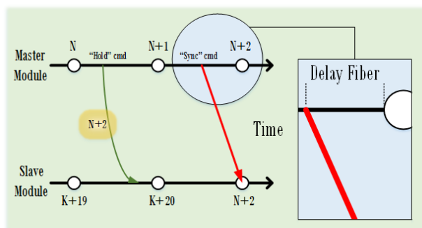
Figure 3: Common time diagram.
