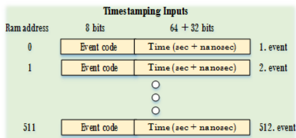
Figure 7: Timestamping input diagram.
