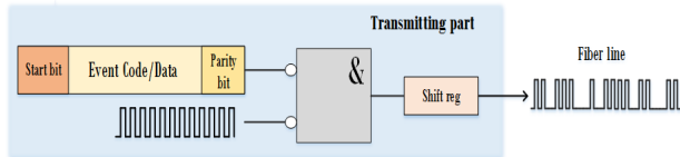
Figure 4: Events transmitting diagram.
