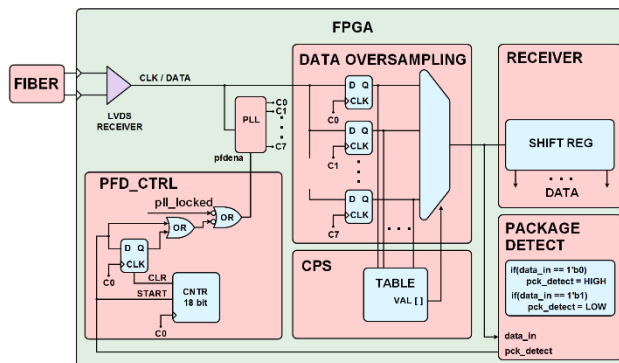
Figure 8: L-Timer detection scheme.
