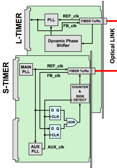
Figure 9: Block diagram of sub-nanosecond phase compensation.
