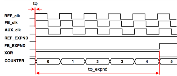
Figure 10: Time diagram of the stroboscopic phase measurement.
