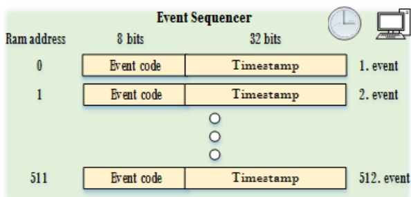
Figure 5: Event Sequencer diagram.
