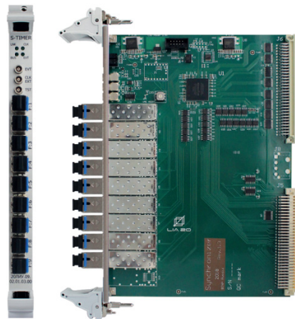
Figure 2: S-Timer module.
