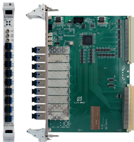
Figure 6: L-Timer module.
