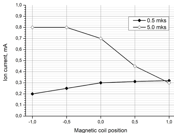
Figure 5: Plot of dependence of the extracted ion current on position of the magnetic coil center about anode: 1 – extreme left position, 0.5 – middle left position, 0 – absence of asperity (the basic case), 0.5 – middle right position, 1 – extreme right position.
