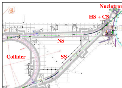
Figure 7: Horizontal projection of the Nuclotron-Collider beam transport channel.
