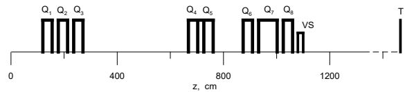
Figure 2: New scheme of the beam line #3. Here Q_{1-8} are quadrupoles, VS is a vertical scanner, T is a target.
