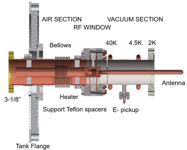
Figure 3: Coupler design for SSR1 RISP cavity.
