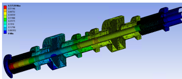
Figure 8: Deformation of the coupler.
