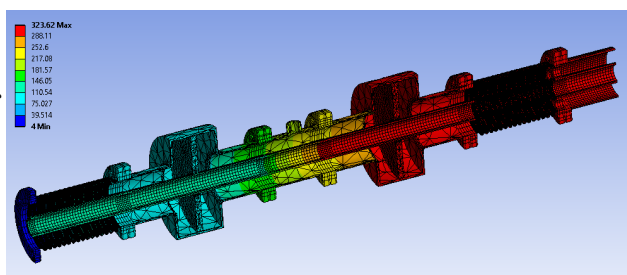
Figure 5: Temperature of the coupler in operation.
