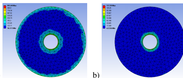
Figure 7: Mechanical stress in the cold (a) and warm (b) windows.
