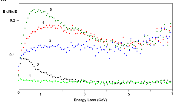
Figure 2: The calculated energy losses: 1) in one 2.5 mm long nonoriented strip; 2) in one strip oriented in planar orientation; 3) in nonoriented multistrip, 4) in single crystal with the thickness 15 mm; 5) multistrip with 6 strips in planar orientation.
