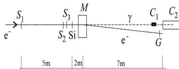
Figure 3: Schematic of the Crystal setup: ( S_1 – S_3 ) scintillation counters, ( C_1 , C_2 ) calorimeters for the determination of the energy of generated photons, (G) hodoscope for the determination of coordinates of electrons behind the magnet and (Si) crystal in goniometer.
