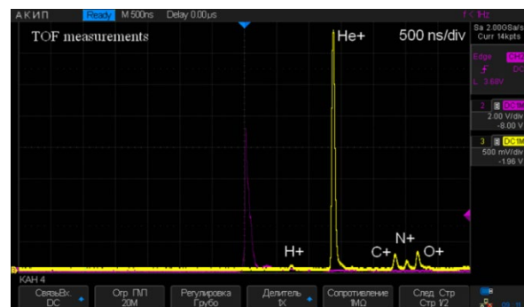
Figure 1: TOF spectrum of the ions at the output of the helium ion source.
