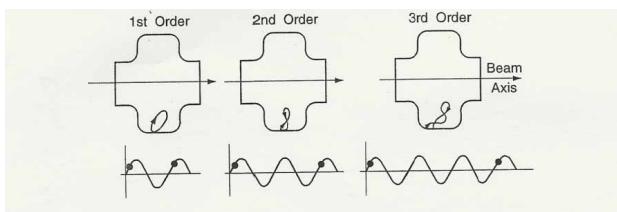
Figure 1: A visualization of 1 st to 3 rd order one-point multipacting, taken from [1]. The order of a multipacting resonance is a measure of the number of
