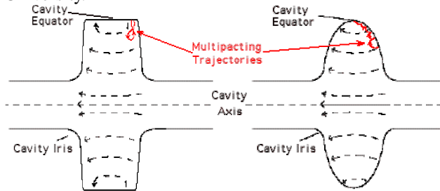
Figure 2: The classic example for a successful geometry change is the HEPL cavity. Single-point multipacting on the flat outside wall led to the preferred use of elliptical cavities for superconducting applications. Figure taken from [5].
