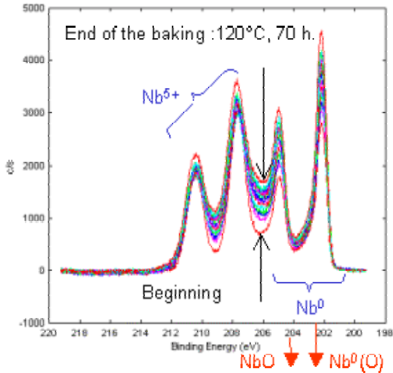
Figure 6: evolution of the Nb signal during a 3 days baking at 120°C. The 2 peaks at the right side correspond to Nb 0 while the 2 peaks at the left side correspond to Nb 5+ ; the apparition of a 3 rd component (Nb 4+ ) can be inferred from the enlargement of the middle of the spectra.
