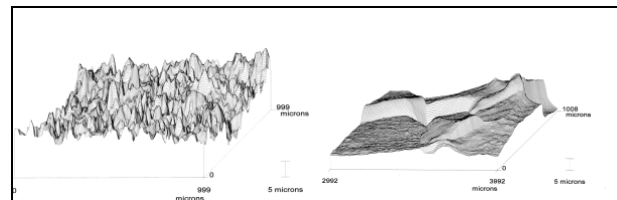
Figure 2 example of variation of surface roughness on 2 Nb samples from the same sheet treated with the same chemical polishing, left: un-annealed, right: annealed sample
