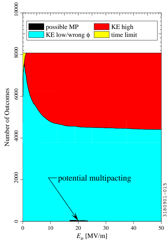
Figure 5. “Pie chart” for multipacting in the APT \beta_g = 0.64 cavity (in the case of K_i = 2 eV and \alpha_i = 0 ). For the majority of initial conditions, the simulation is ended when the K_f falls below 20 eV; for most other cases, K_f ultimately exceeds 3 keV. There is one multipacting band (black region at bottom).
