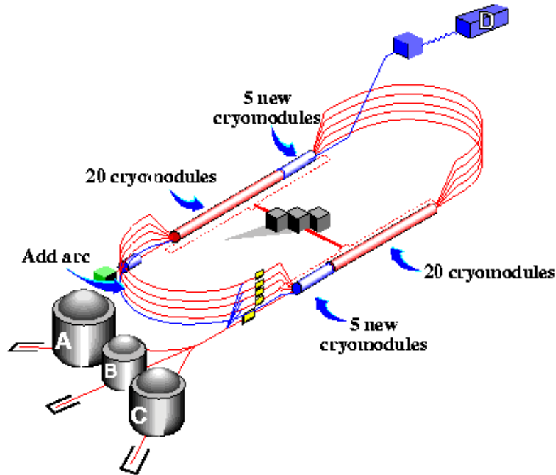
Figure. 1 Illustration of the concept for upgrading CEBAF to 12 GeV
