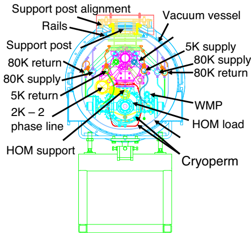
Figure 2: Transverse 2D cross section of the ERL injector module.
