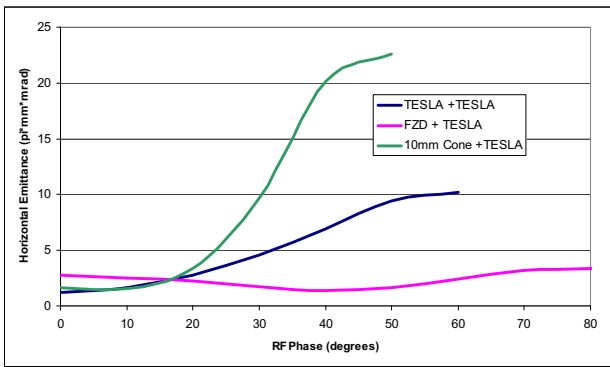
Figure 8: RMS transverse emittance as a function of RF phase
