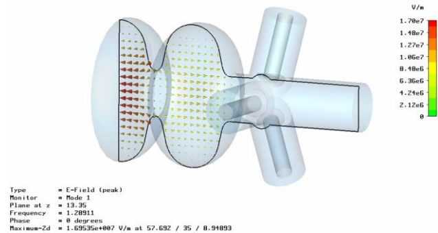
Figure 7: Electric field contours in a TESLA 1½ cell cavity
