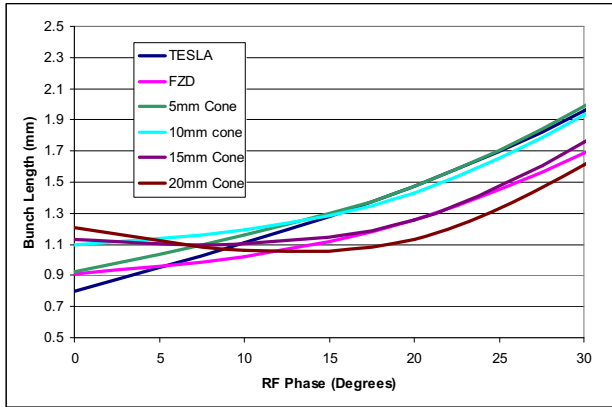
Figure 4: Comparison of bunch length for half-cell cavities
