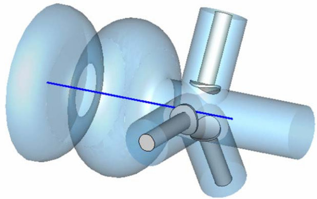
Figure 1: Conceptual design of 1½ cell gun cavity with fundamental power couplers located at 120°
