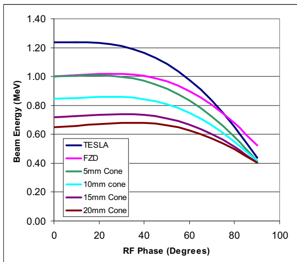
Figure 5: Beam Energy as a function of RF phase for each cavity assessed
