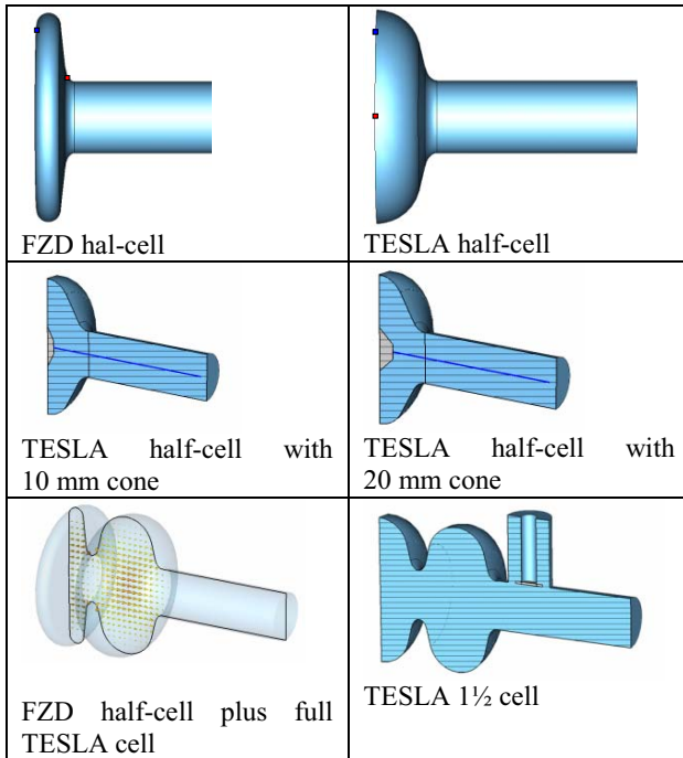
Figure 2: RF design of the first 1/2 cell and complete cavities that have been assessed
