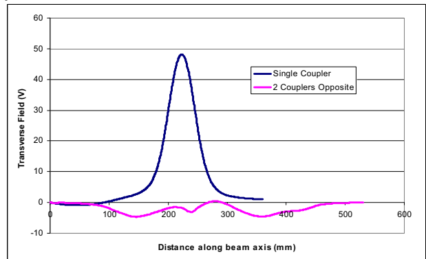
Figure 3: Transverse electric fields in the coupler’s region
