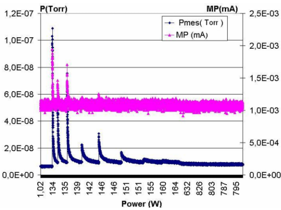
Figure 9: Multipacting and vacuum measurement versus RF power
