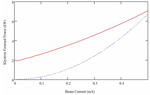
Figure 4: CEBAF 12GeV, LL cavity's klystron power (red) and beam power (blue) verse beam current at Eacc=20MV/m.
