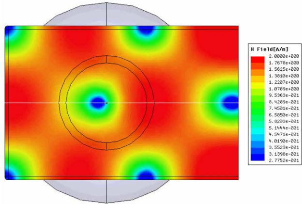
Figure 1: Magnetic field amplitude in coupler center plane.
