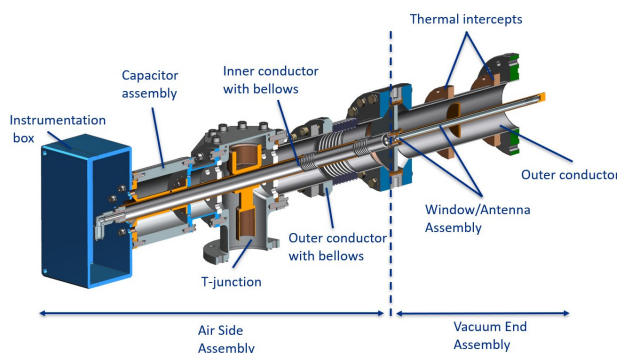
Figure 11: Cut-view of 325 MHz PIP-II coupler.
