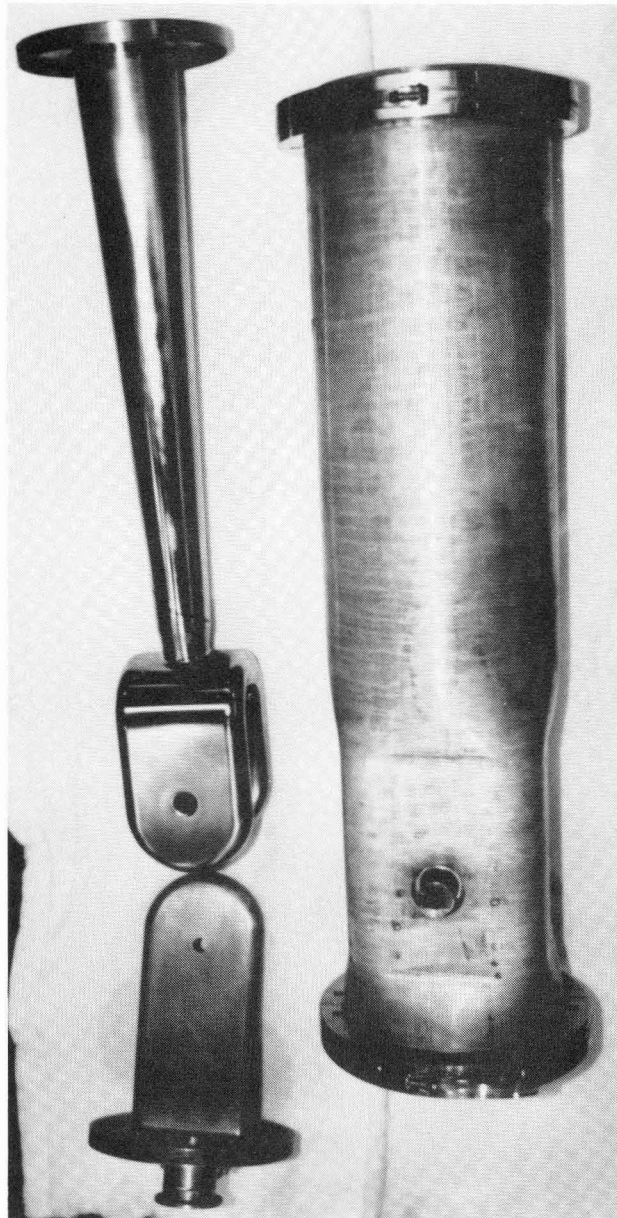
Figure 3. Elements of the prototype I3 resonator prior to final welding and assembly. Pieces shown include the explosively-bonded Nb-Cu outer housing, the high-purity niobium center conductor and forked drift-tube, and the demountably joined counter drift tube.
