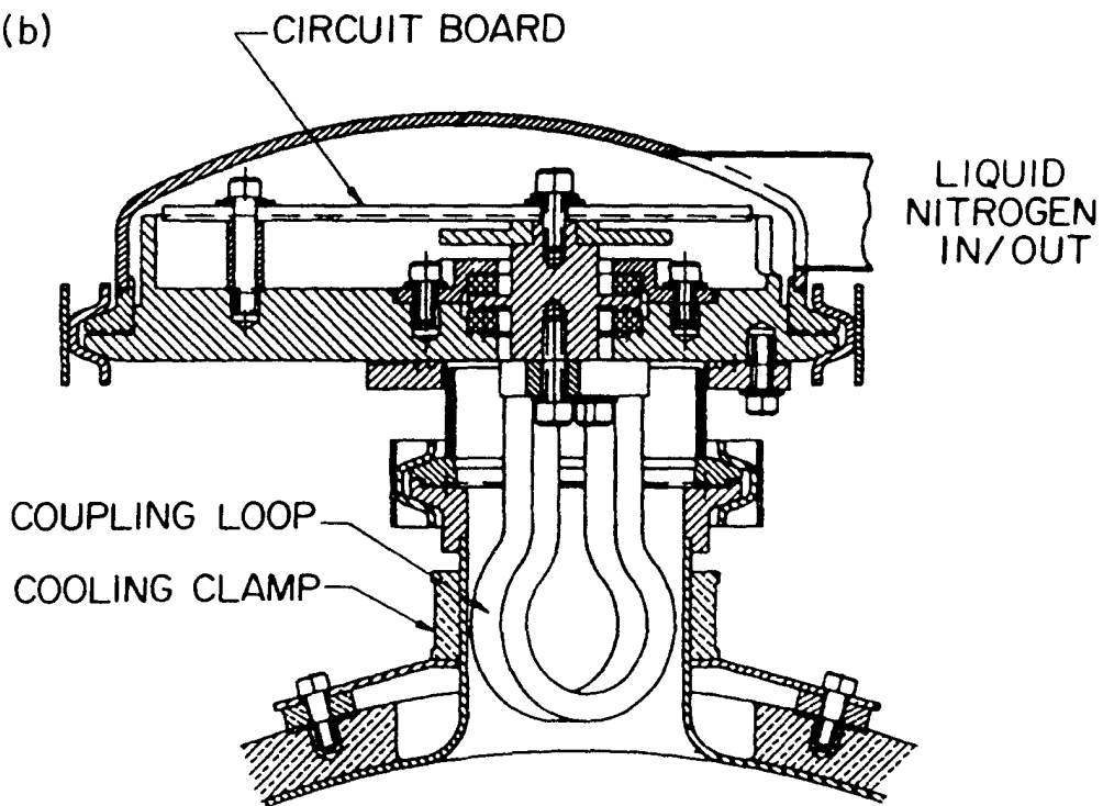
Figure 1. Two versions of the fast tuning system required to control the phase of ATLAS resonators. The first version (a) was capacitively coupled. Currently being developed is an inductively coupled version (b).
